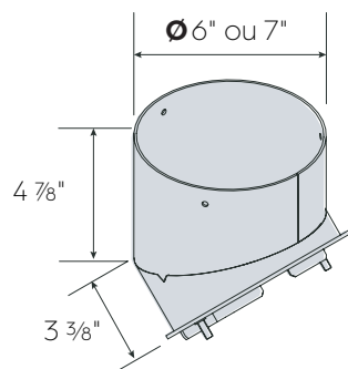
VERTICAL | 90° Ø 6" 12020001 Ø 7" 12002005
